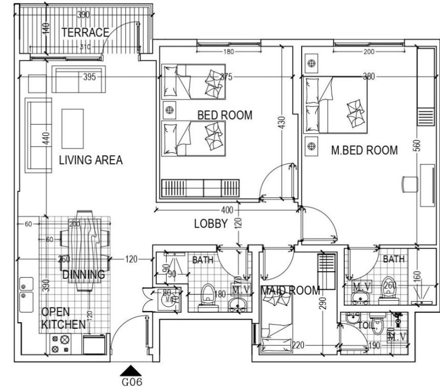
FLAT=G06 (AREA 109.00 M2) 2 BED ROOM/LIVING /DINNING TERRACE/COM.BATH/KITCHEN/MAID ROOM+TOILET
