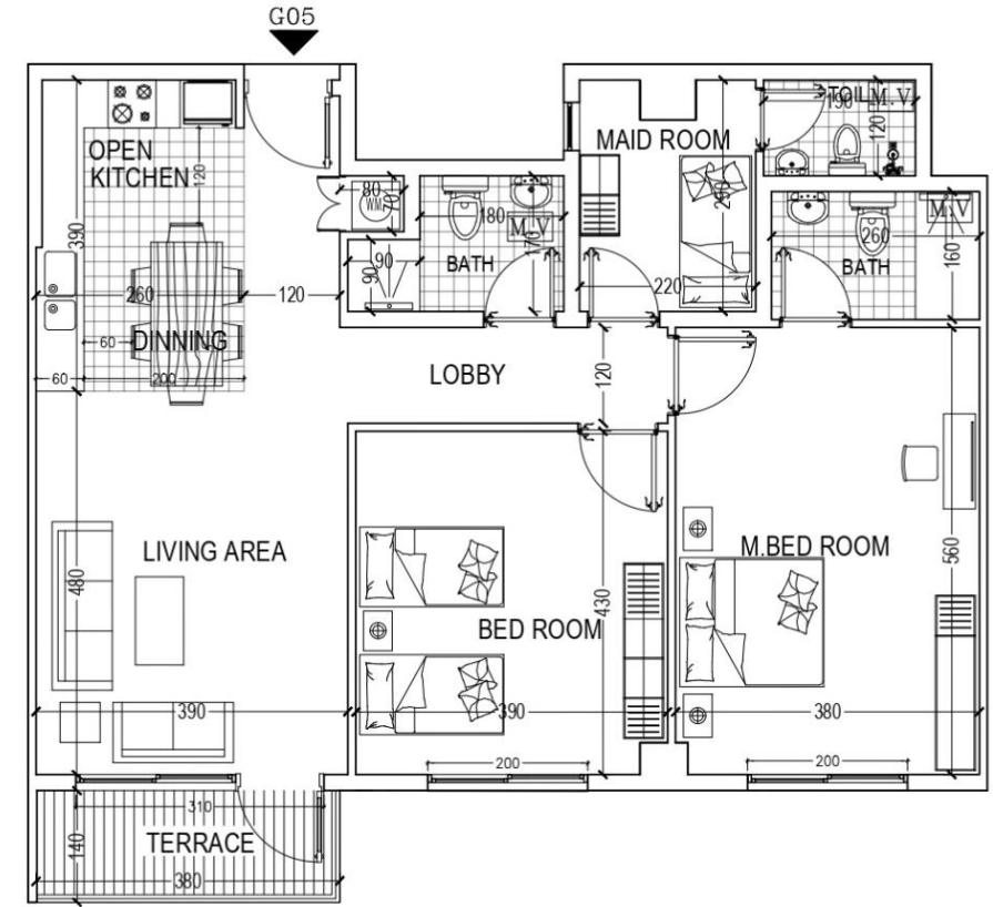
FLAT=G05 (AREA 110.60 M2) 2 BED ROOM/LIVING /DINNING TERRACE/COM.BATH/KITCHEN/MAID ROOM+TOILET
