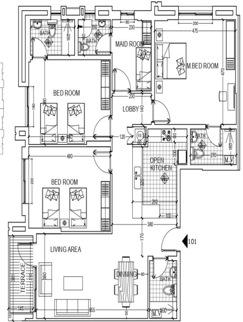
FLAT=101 (AREA160.00 M2) 3 BED ROOM/LIVING /DINNING TERRACE/COM.BATH/KITCHEN/MAID ROOM+TOILET
