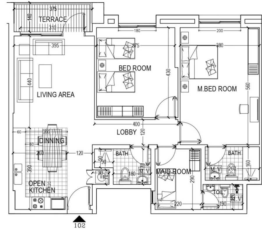
FLAT=102 (AREA 112.90 M2) 2 BED ROOM/LIVING /DINNING TERRACE/COM.BATH/KITCHEN/MAID ROOM+TOILET
