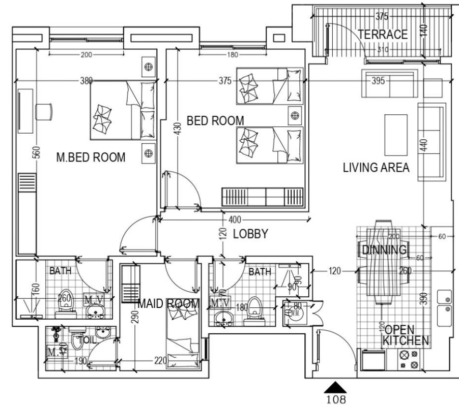
FLAT=108 (AREA 112.90 M2) 2 BED ROOM LIVING /DINNING TERRACE/COM.BATH/KITCHEN/MAID ROOM+TOILET
