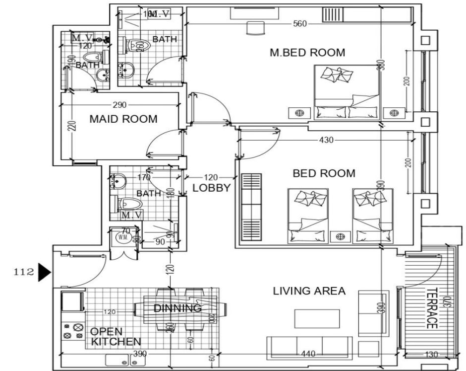
FLAT=112 (AREA 111.00 M2) 2 BED ROOM/LIVING /DINNING TERRACE/COM.BATH/KITCHEN/MAID ROOM+TOILET
