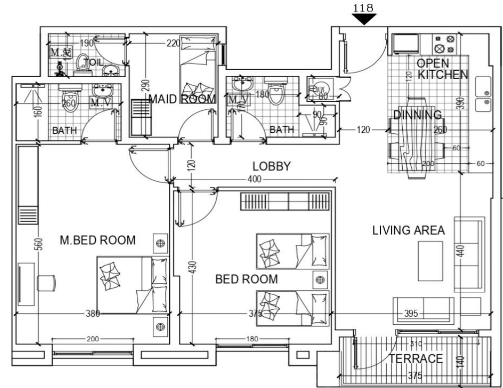
FLAT=118 (AREA 112.90 M2) 2 BED ROOM LIVING /DINNING TERRACE/COM.BATH/KITCHEN/MAID ROOM+TOILET
