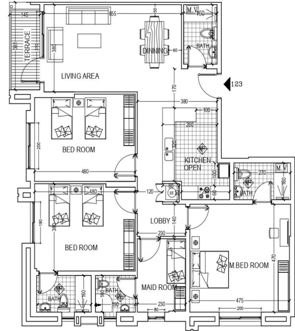
FLAT=123 (AREA160.00 M2) 3 BED ROOM/LIVING /DINNING TERRACE/COM.BATH/KITCHEN/MAID ROOM+TOILET
