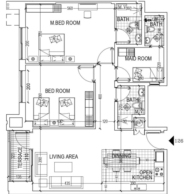
FLAT=126 (AREA 112.00 M2) 2 BED ROOM/LIVING /DINNING TERRACE/COM.BATH/KITCHEN/MAID ROOM+TOILET
