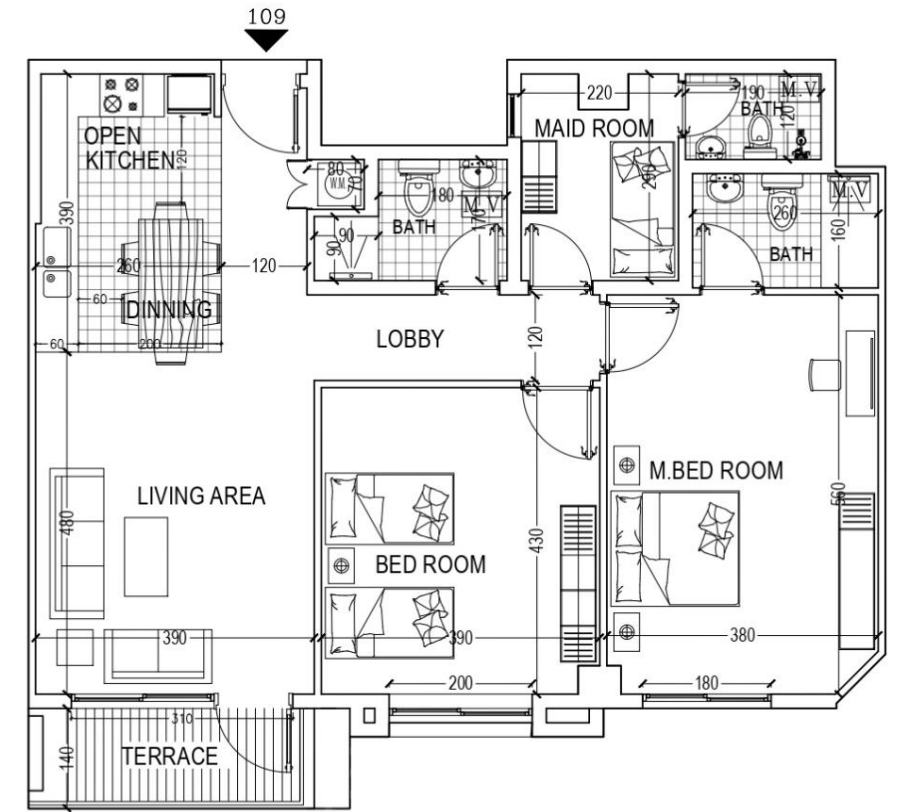
FLAT=109 (AREA 112.15 M2) 2 BED ROOM LIVING /DINNING/ TERRACE/COM.BATH/KITCHEN/MAID ROOM+TOILET
