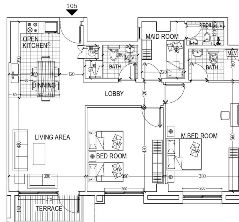
FLAT=105 (AREA 113.60 M2) 2 BED ROOM/LIVING /DINNING TERRACE/COM.BATH/KITCHEN/MAID ROOM+TOILET
