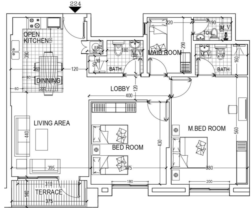
FLAT=224 (AREA 112.90 M2) 2 BED ROOM/LIVING /DINNING TERRACE/COM.BATH/KITCHEN/MAID ROOM+TOILET
