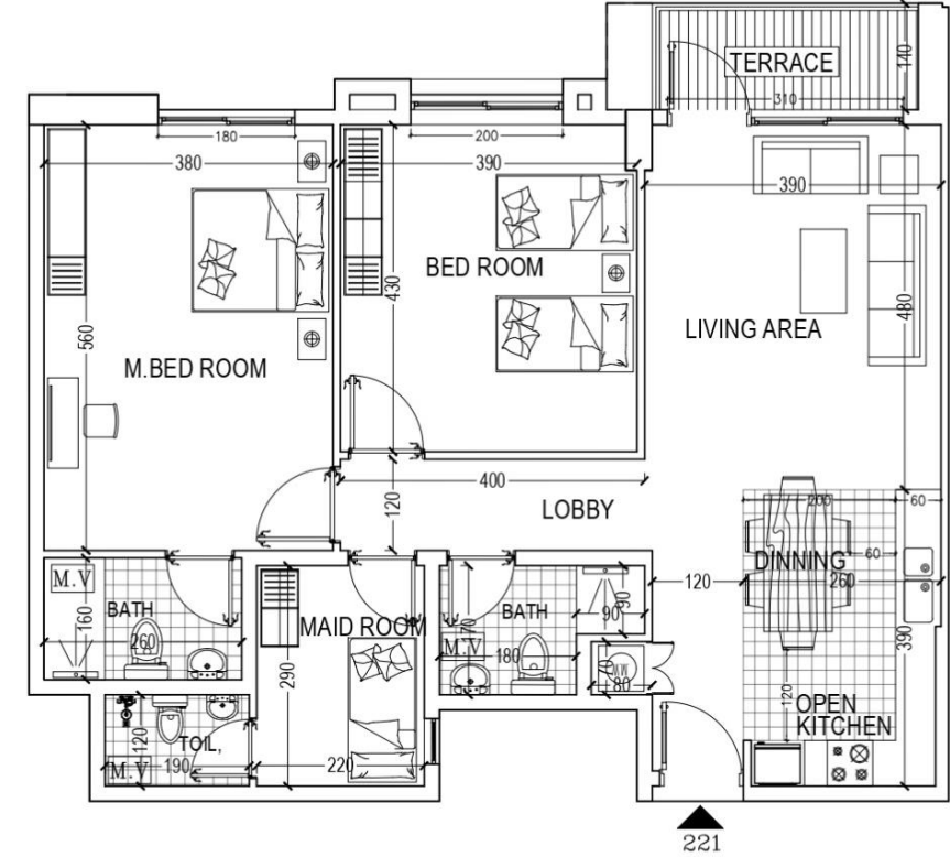
FLAT=221 (AREA 113.60 M2) 2 BED ROOM/LIVING /DINNING/ TERRACE/COM.BATH/KITCHEN/MAID ROOM+TOILET
