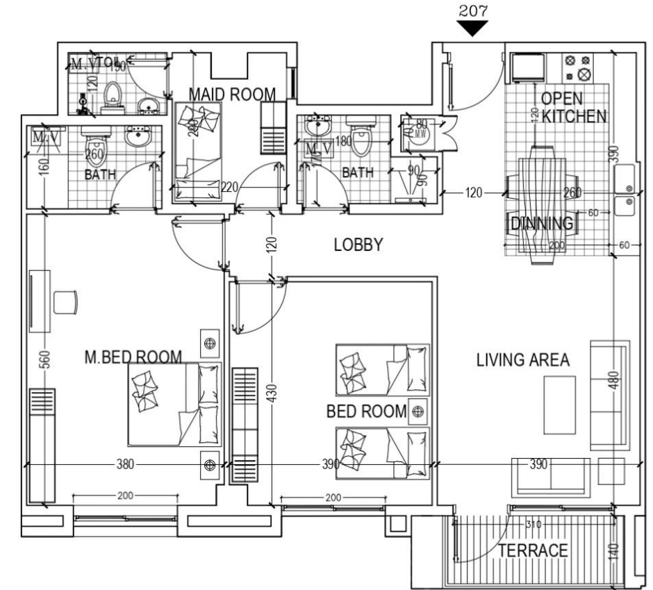
FLAT-207 (AREA 113.60 M2) 2 BED ROOM/LIVING /DINNING TERRACE/COM.BATH/KITCHEN/MAID ROOM+TOILET
