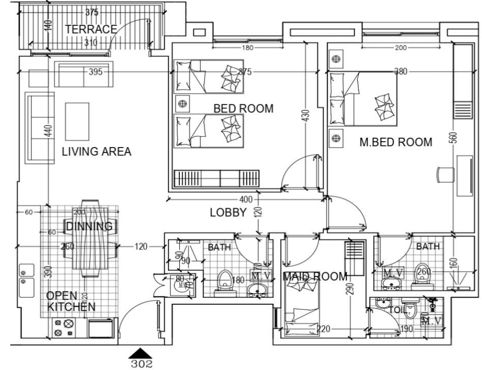
FLAT=302 (AREA 112.90 M2) 2 BED ROOM/LIVING /DINNING TERRACE/COM.BATH/KITCHEN/MAID ROOM+TOILET
