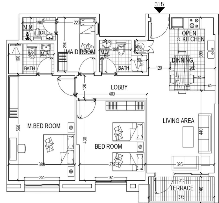
FLAT=318 (AREA 112.90 M2) 2 BED ROOM LIVING /DINNING TERRACE/COM.BATH/KITCHEN/MAID ROOM+TOILET
