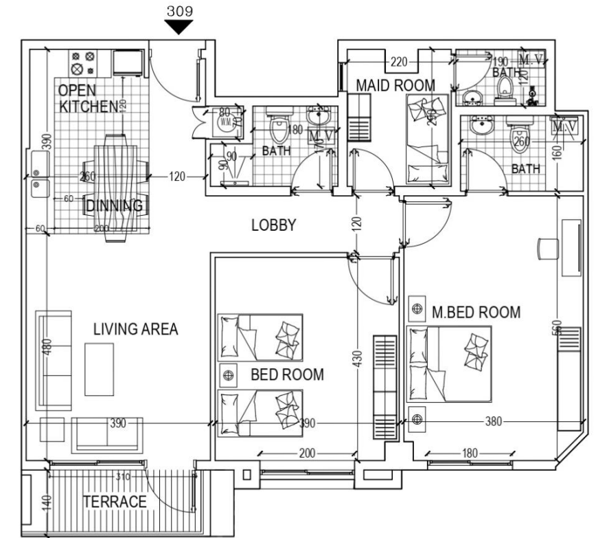
FLAT=309 (AREA 112.15 M 2 ) 2 BED ROOM LIVING /DINNING/ TERRACE/COM.BATH/KITCHEN/MAID ROOM+TOILET
