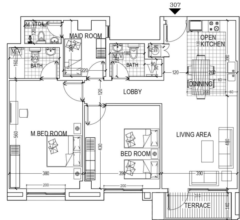
FLAT-307 (AREA 113.60 M2) 2 BED ROOM/LIVING /DINNING TERRACE/COM.BATH/KITCHEN/MAID ROOM+TOILET
