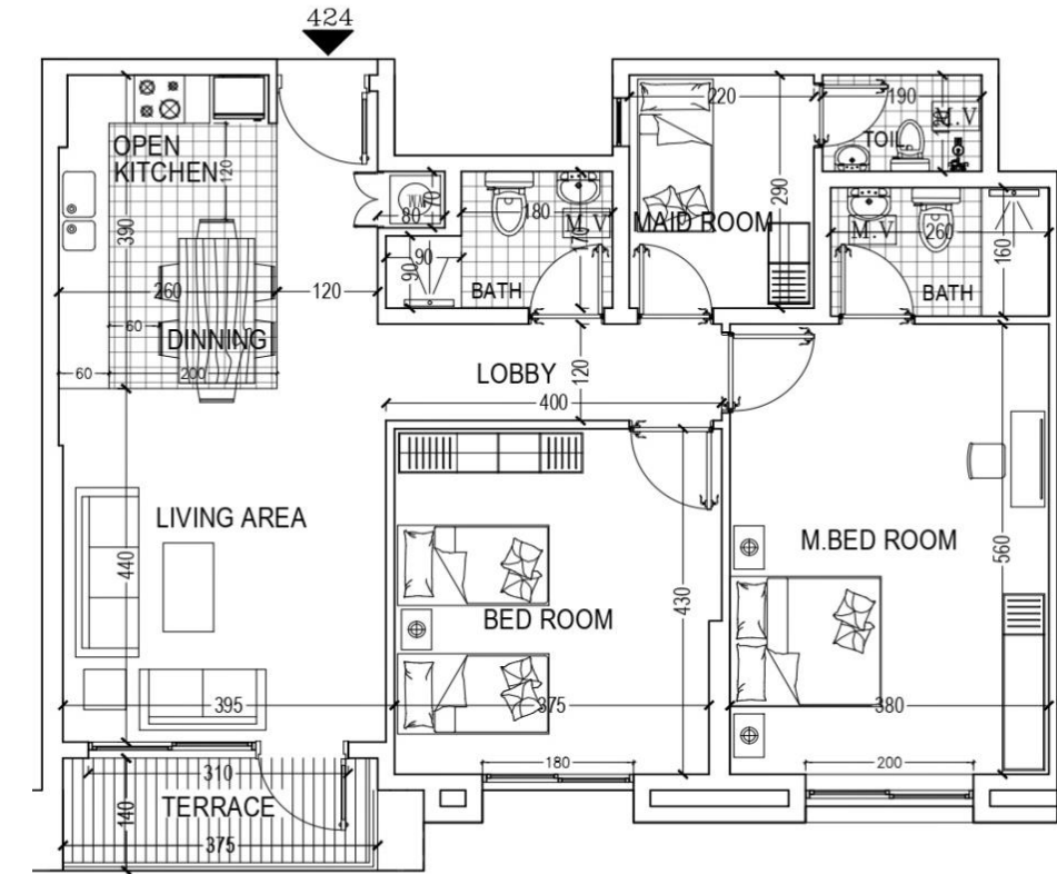
FLAT=424 (AREA 112.90 M2) 2 BED ROOM/LIVING /DINNING TERRACE/COM.BATH/KITCHEN/MAID ROOM+TOILET
