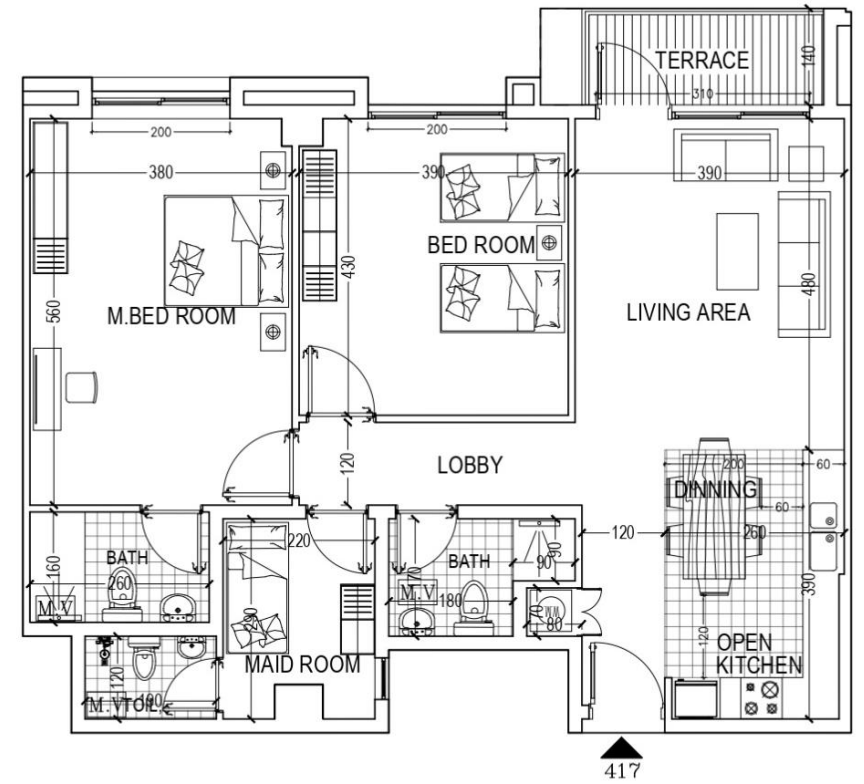
FLAT-417 (AREA 113.60 M2) 2 BED ROOM/LIVING /DINNING
