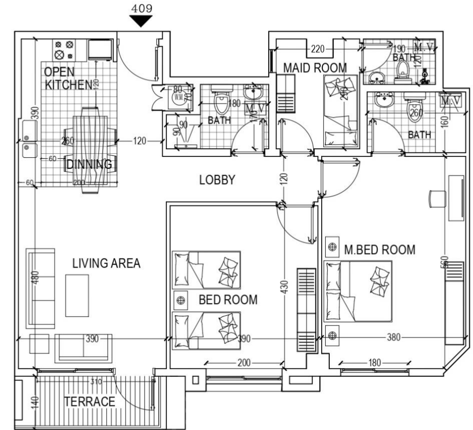
FLAT=409 (AREA 112.15 M2) 2 BED ROOM LIVING /DINNING/ TERRACE/COM.BATH/KITCHEN/MAID ROOM+TOILET
